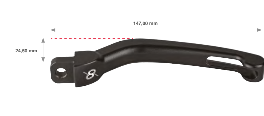
Aluminium half lever "Standard" (RH/LH) - Leva in alluminio "Standard"(DX/SX) - cod. LL05
